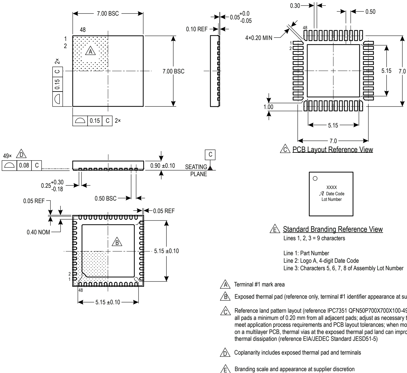
Figure 5: Package EV, 48 Terminal Wettable Flank QFN with Exposed Thermal Pad
