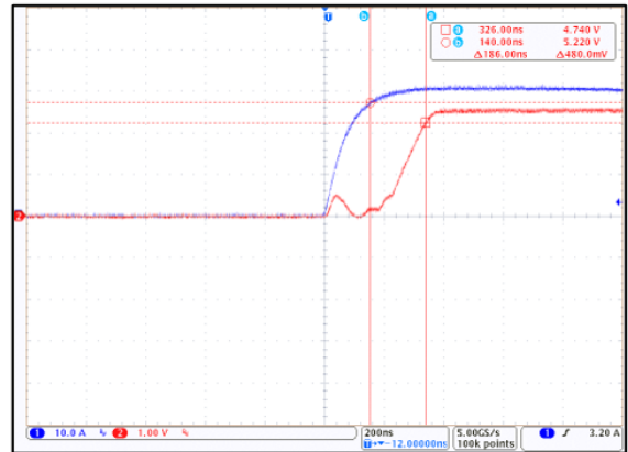
Figure 9: CT425 Response Time; I_P = 30\ \text{A}_{PK} and C_L = 100\ \text{pF} (Blue = I_{CC} , Red = V_{OUT} )
