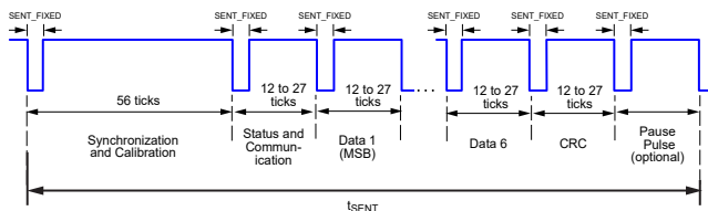
Figure 1: SENT Message Structure
