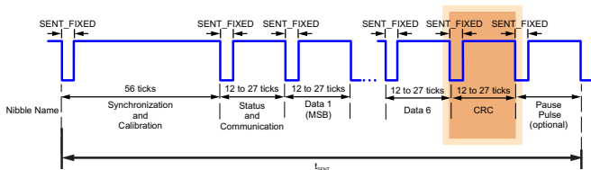
Figure 5: CRC Nibble
