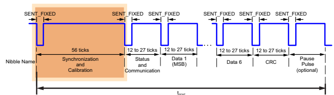
Figure 2: Synchronization and Calibration Nibble
