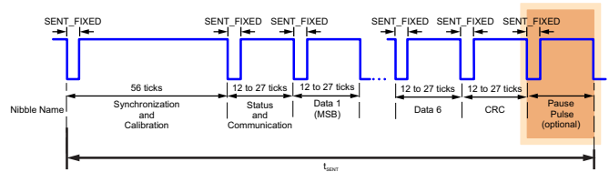
Figure 6: Pause Pulse
