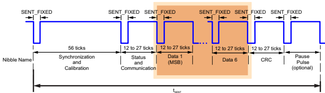
Figure 4: Data Nibble
