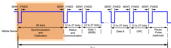
Figure 3: Status and Communication Nibble
