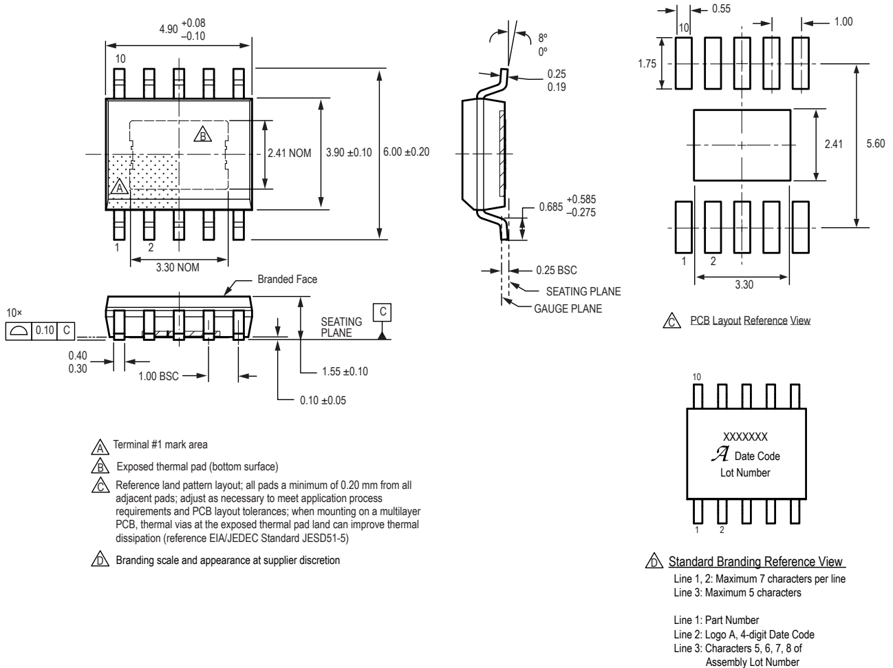
Figure 19: Package LK, 10-Pin SOIC with Exposed Thermal Pad
