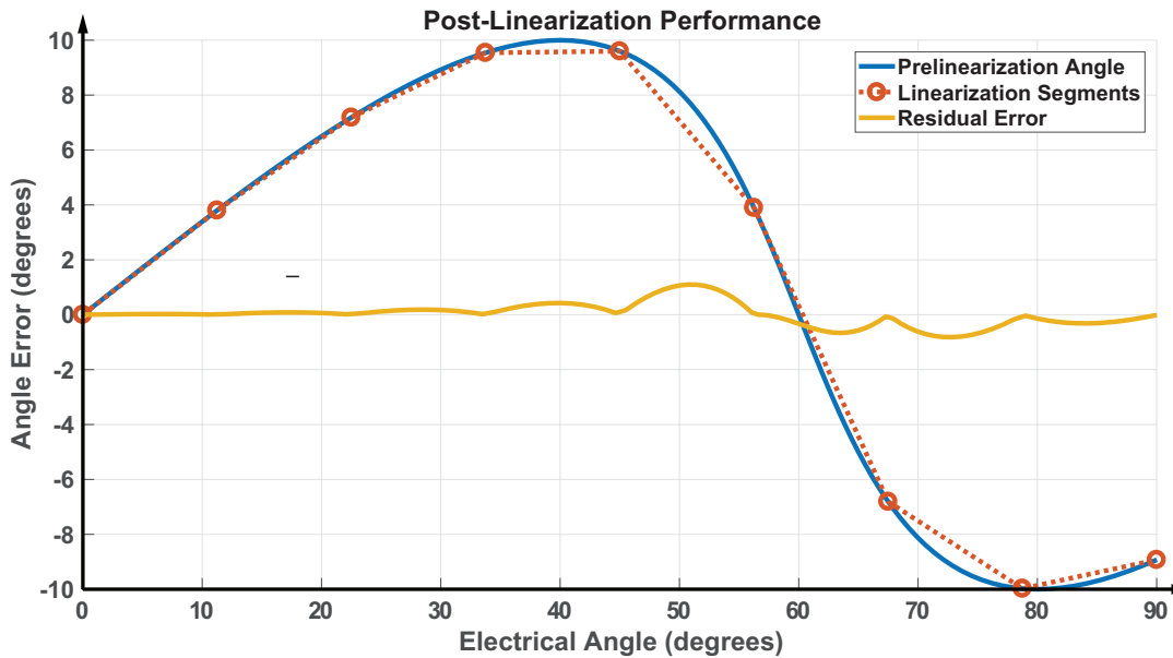
Figure 8: Post-Linearization Error
