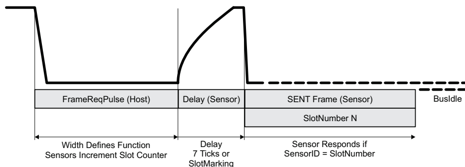
Figure 47: SSENT Sensor Addressing
