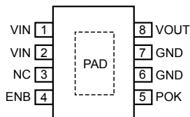
Pinout Diagram
