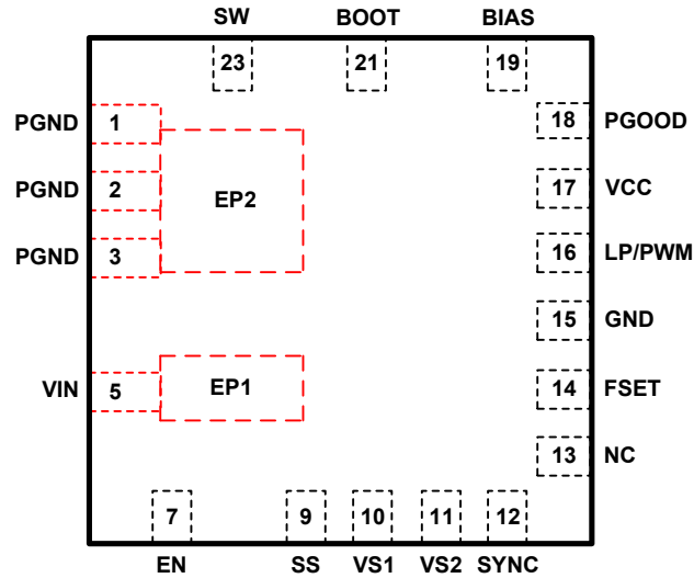
Figure 2: QFN-24 Pinout Diagram—24-Pin 4 mm × 4 mm × 2.1 mm Wettable Flank QFN Package
