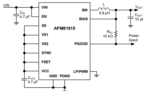
Figure 1: APM81815 Typical Application Circuit
