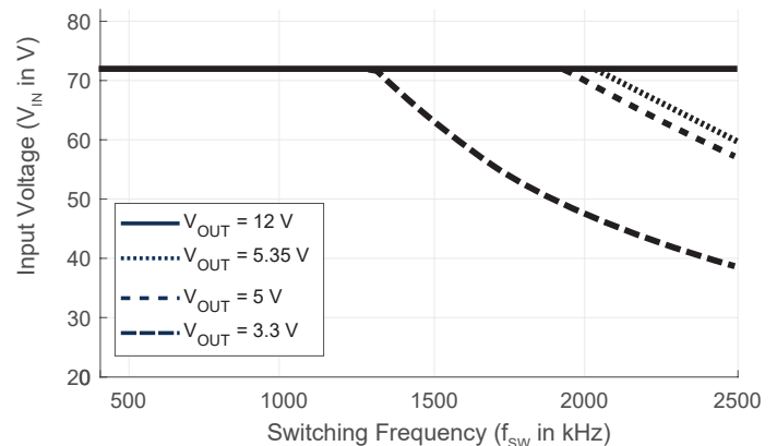
Figure 8: Input Voltage Limit to Prevent Pulse-Skipping Measured at I_{OUT} = 100 mA
