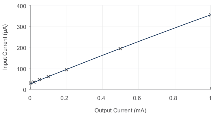
Figure 7: Low-Power Mode Input Current ( V_{IN} = 48 V, V_{OUT} = 12 V, L = 6.8 \mu H)
