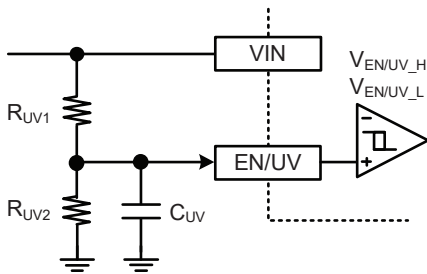
Figure 10: Input Undervoltage Lockout with EN Pin
