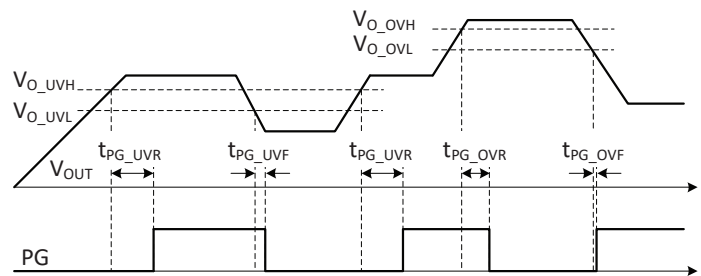
Figure 11: Power Good Operation
