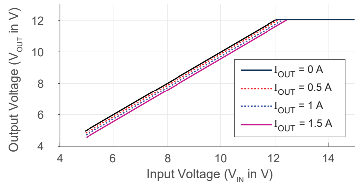
Figure 9: 12 V Output Voltage Dropout at Low V_{IN}
