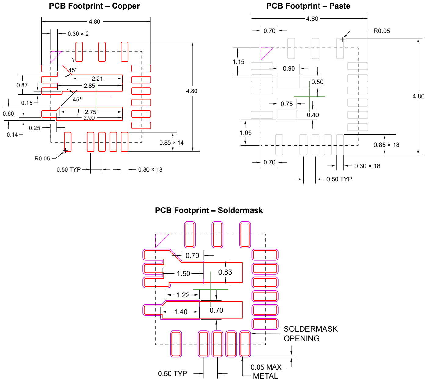
Figure 14: Recommended PCB Footprint
