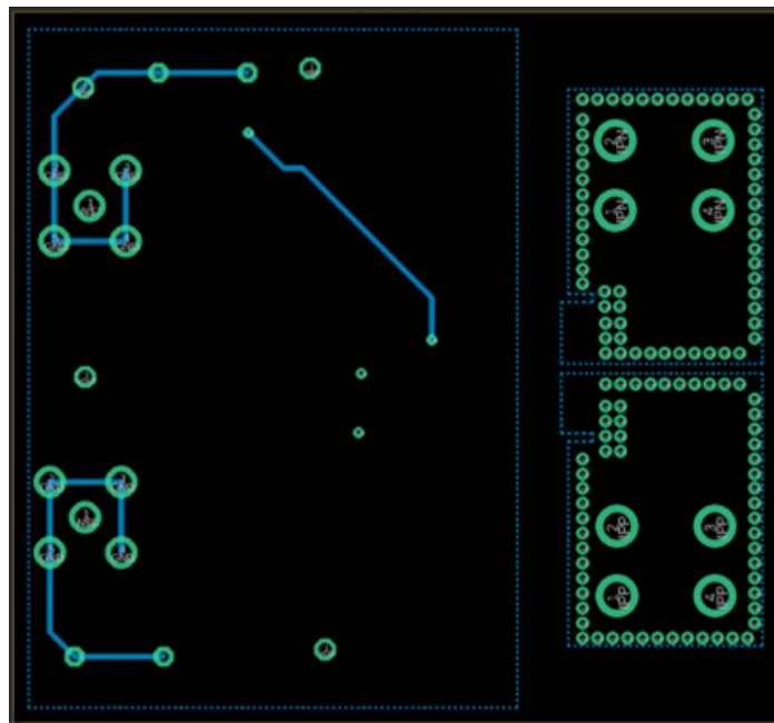
Figure 5: Bottom Layer
