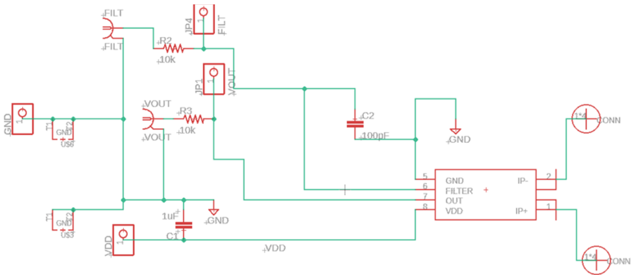
Figure 3: CT416-20AC Evaluation Board Schematic
