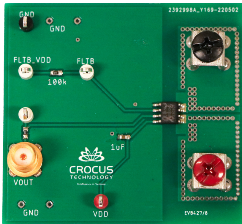
Figure 2: CT427-50AC Evaluation Board
