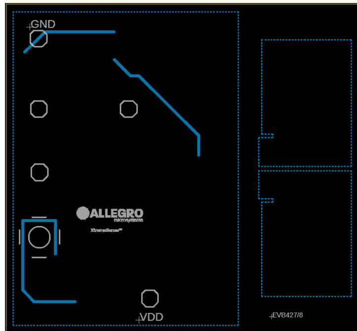
Figure 5: Bottom Layer
