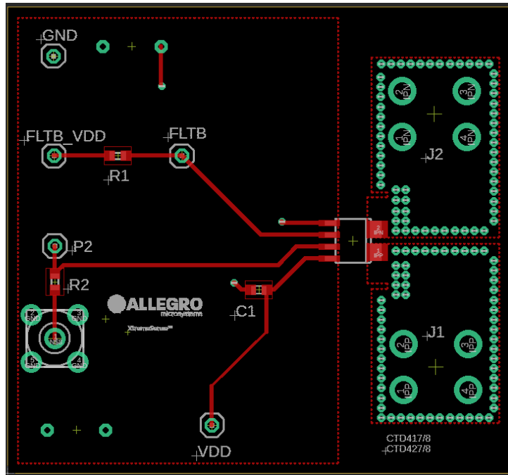
Figure 4: Top Layer
