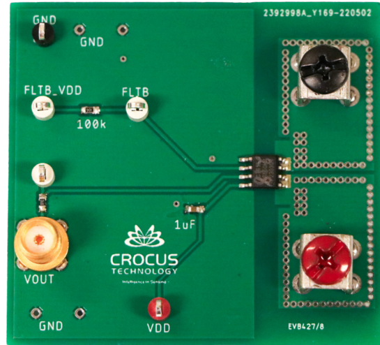
Figure 1: CT427-50AC Evaluation Board
