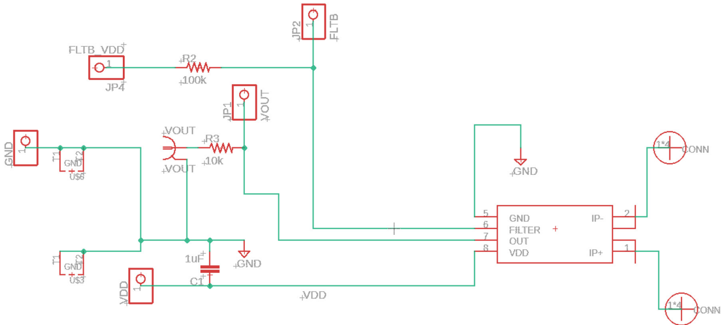
Figure 3: CT427-50AC Evaluation Board Schematic
