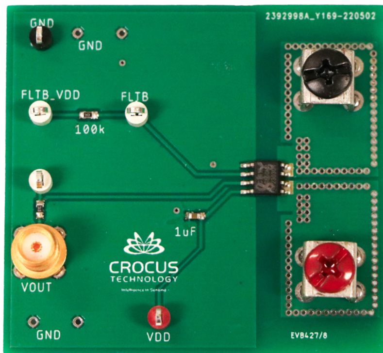
Figure 2: CT428-20AC Evaluation Board
