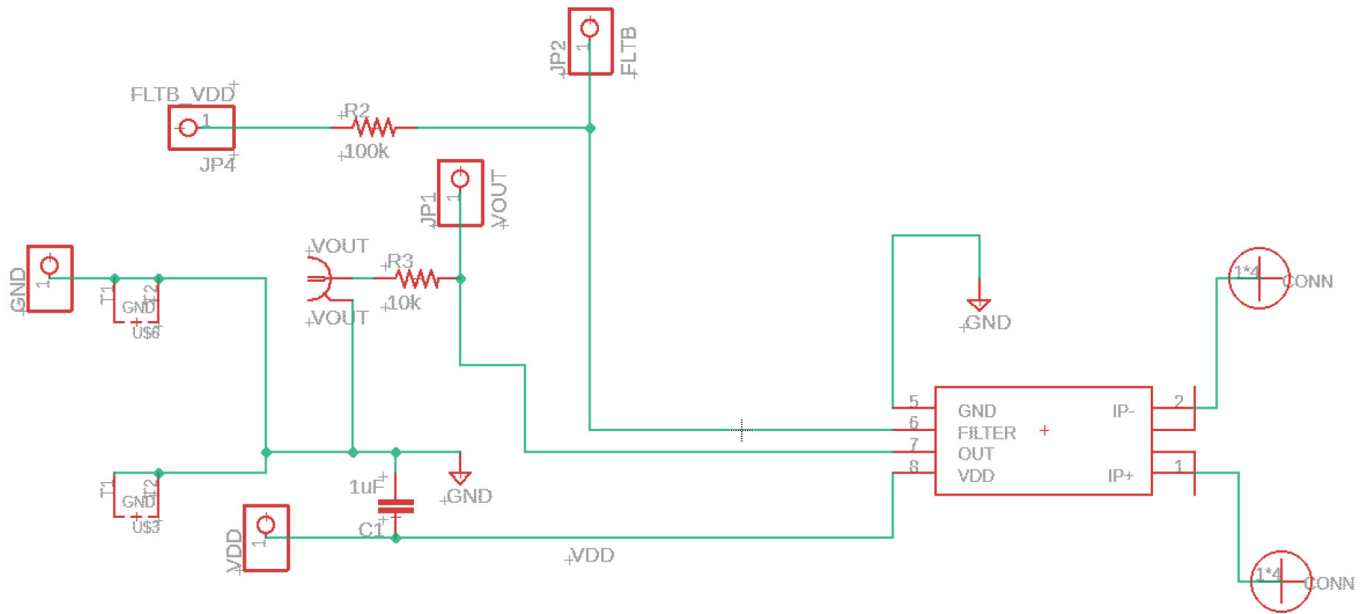
Figure 3: CT428-20AC Evaluation Board Schematic
