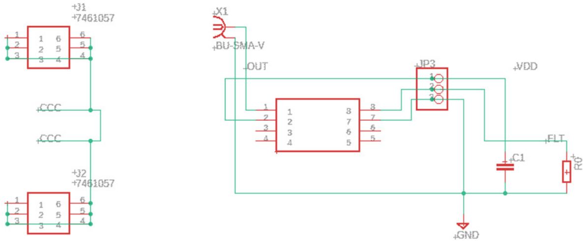
Figure 3: CTD455-BB-06B5 Schematic
