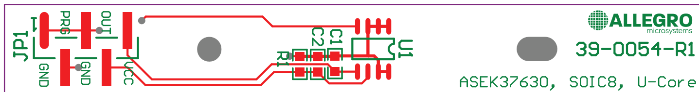
Figure 6: PCB Layout (Top Layer)
