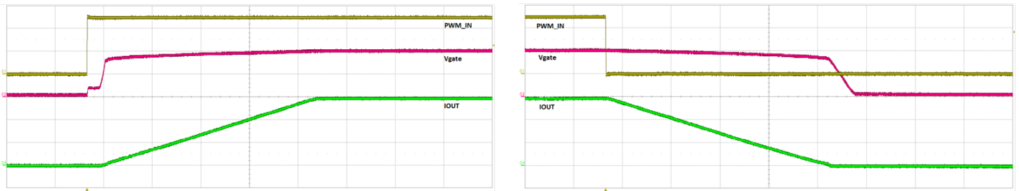
Figure 16: Rise Time and Fall Time During PWM Dimming. I_{OUT} (Total LED Current) (200 mA/div), PWM_IN and V_{GATE} (2 V/div), Time (20 \mu s/div)
