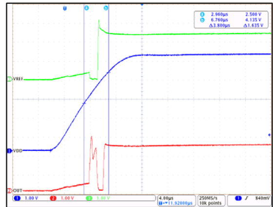
Figure 10: CT452 Startup Waveforms for V_{OQ} = 2.50\text{ V} (Bipolar Sensor Variant)
