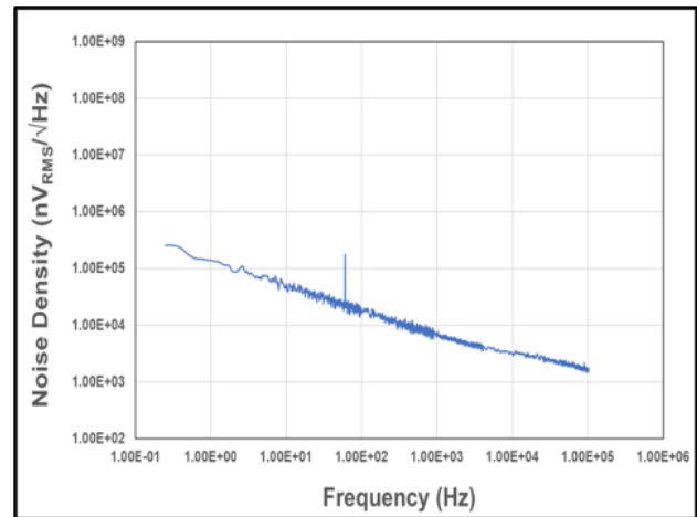
Figure 14: Noise Density vs. Frequency
