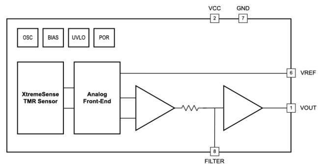
Figure 2: CT452 Functional Block Diagram for TSSOP-8
