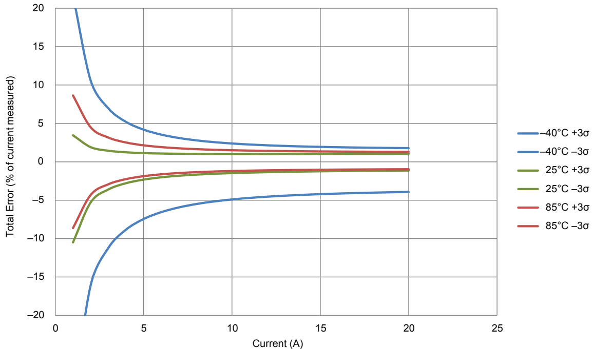
Figure 3: Predicted Total Error as a Function of Sensed Current for the ACS725KMATR-20AB
