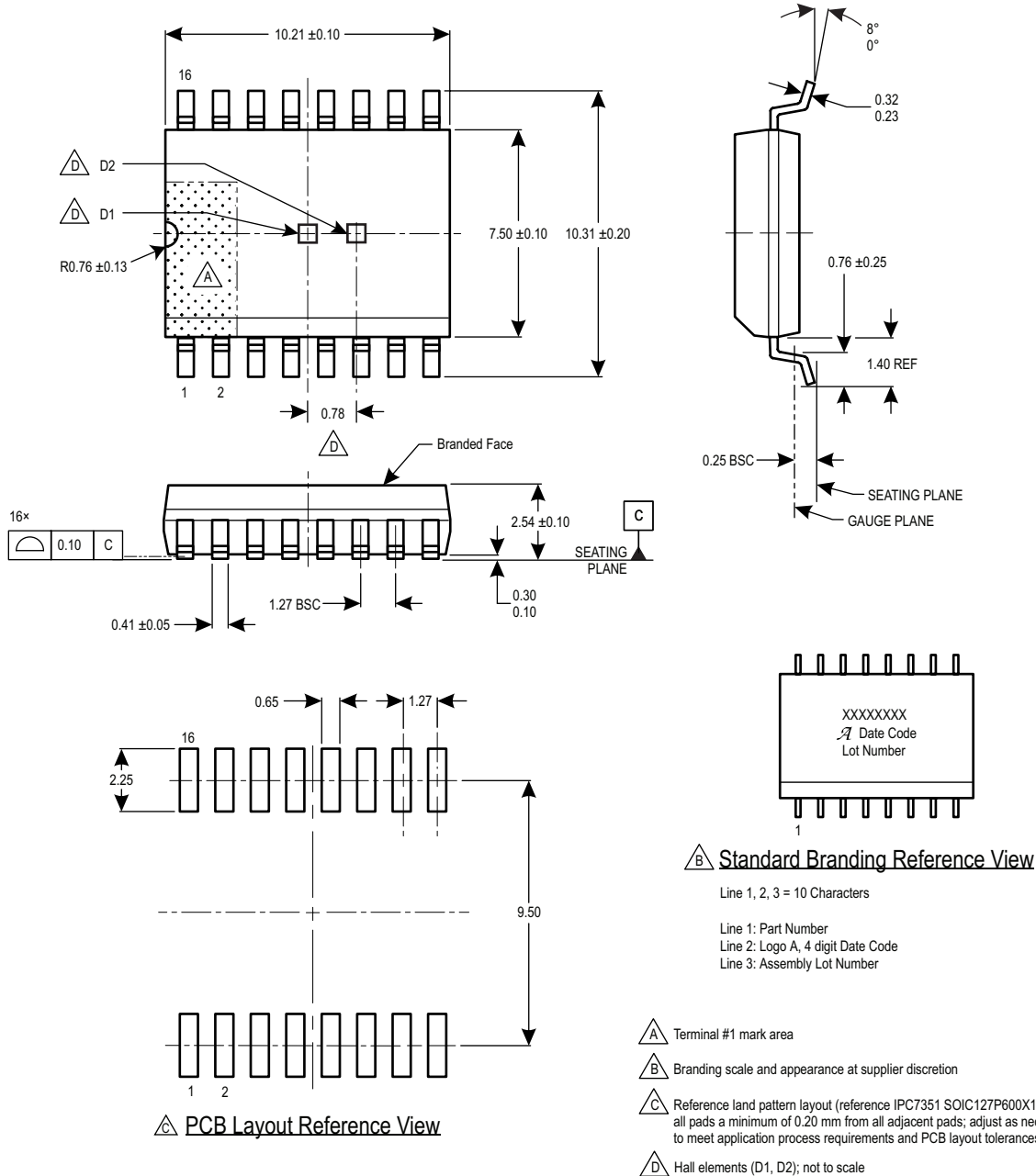
Figure 9: Package MA, 16-Pin SOICW
