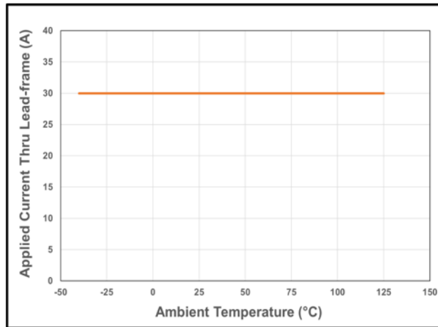
Figure 22: CT427 Current Derating Curve for 30 A DC
