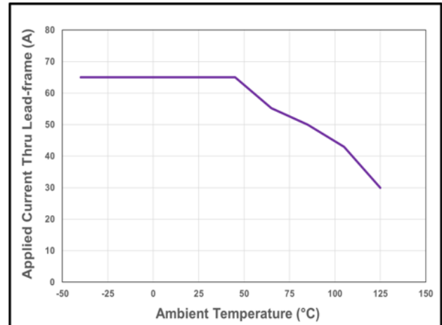
Figure 29: CT433 Current Derating Curve for 65 A DC
