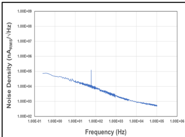
Figure 28: Noise Density vs. Frequency
