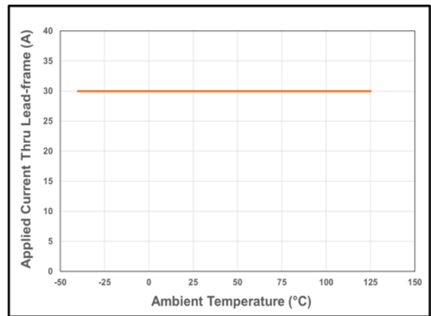
Figure 16: CT433 Current Derating Curve for 30 A DC
