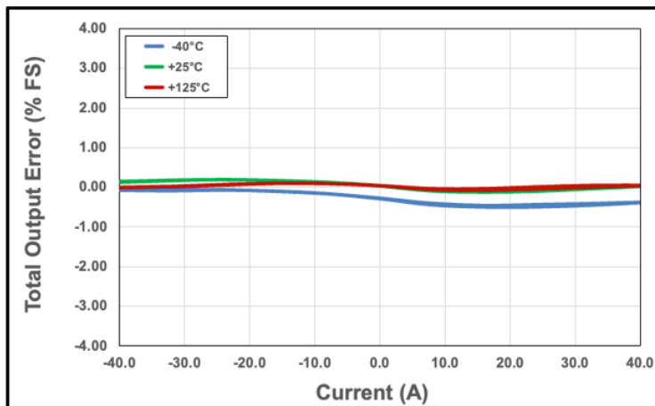
Figure 20: Total Output Error vs. Current vs. Temperature
