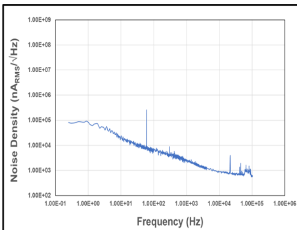
Figure 25: Noise Density vs. Frequency
