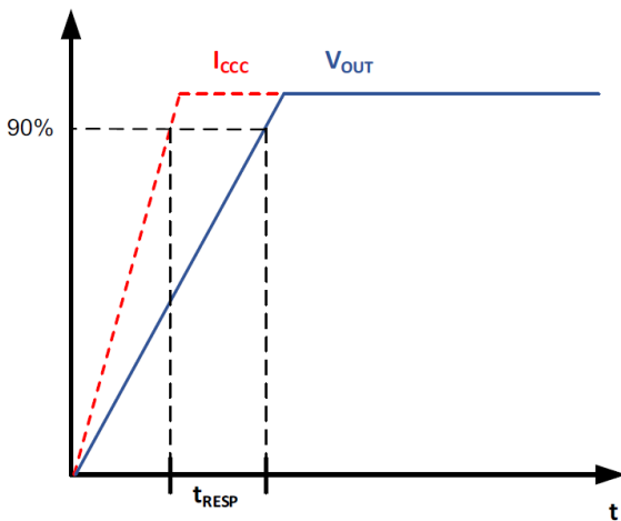
Figure 37: CT433 Response Time Curve
