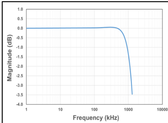
Figure 4: CT433 Bandwidth
