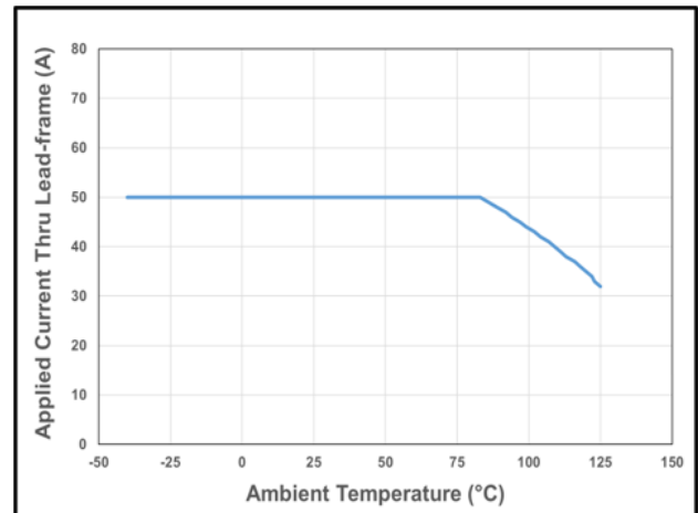
Figure 23: CT433 Current Derating Curve for 50 A DC
